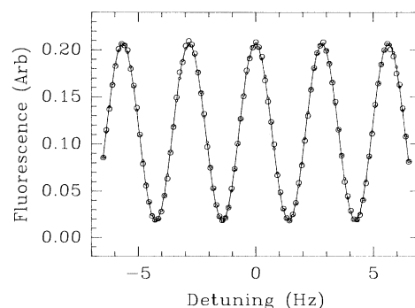
FIG. 3. The central Ramsey fringes of the F=3, m_F=0 \rightarrow F=4, m_F=0 transition. The FWHM linewidth is 1.41 Hz for a fountain height of 15 cm. The large circles are the data (1 launch per point, 0.933 s per launch) and the small circles and line represent the fit to the data.
