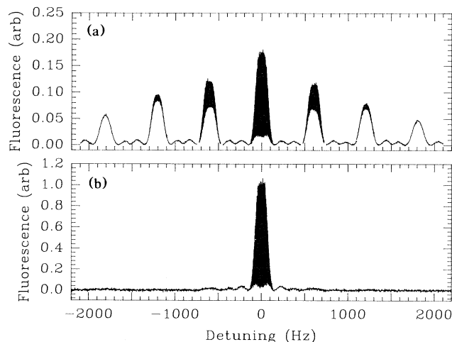
FIG. 2. (a) Clock spectrum of the 7 \Delta m_F = 0 transitions from the F=3, m_F ground-state hyperfine level to the F=4, m_F ground state and (b) the spectrum for 95% of the atoms initially prepared in the F=3, m_F=0 state. The degeneracy of the m_F levels is removed by an 860 \mu G magnetic field.
