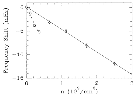
FIG. 4. Frequency shift vs ultracold Cs density for atoms evenly distributed among the F=3, m_F states (solid line) and for atoms in only the m_F=0 states (dashed line). For a density of (1.0 \pm 0.6) \times 10^9 \text{ cm}^{-3} , the shifts are -4.8 \pm 0.2 and -15.8 \pm 1.4 \text{ mHz} .
