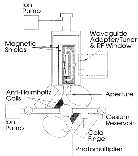
FIG. 1. Fountain schematic. Atoms are trapped in the lower vacuum chamber and launched through the microwave cavity in the upper chamber. Both chambers are pumped by 8 l/s pumps and are separated by a 1.1 cm diam aperture. Microwaves are coupled to the cavity through a coaxial cable connected to the waveguide adapter or tuner and a ceramic vacuum window.
