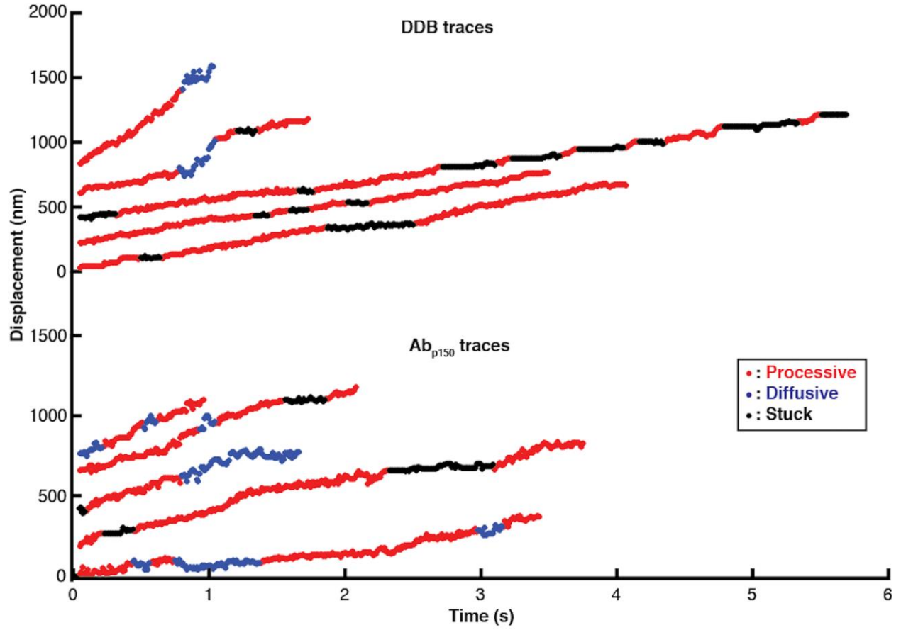
Figure 5. High-resolution DDB tracking and motility state identification. Sample traces of control DDB (top) and DDB in presence of Ab_{p150} (bottom) taken at 100 frames/s by iSCAT microscopy and processed with the state switching algorithm. Processive segments are labeled in red, diffusive episodes in blue, and stuck durations in black.
