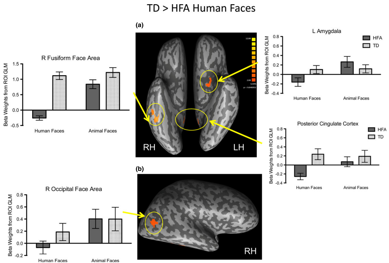
Figure 2 Group differences for HFA adolescents and TD adolescents in response to human faces compared to objects. The maps were generated by computing a whole-brain analysis, corrected at p < .05 . Adolescents with HFA exhibited less activation than TD adolescents for human faces compared to objects in the left putamen (not pictured), (a) right fusiform face area, left amygdala, posterior cingulate cortex, and (b) the right occipital face area. The mean (SEM) beta weight difference scores (human faces minus objects) and (animal faces minus objects) were extracted from these regions. Adolescents with HFA show hypo-activation for human faces, but not animal faces, in these regions.
